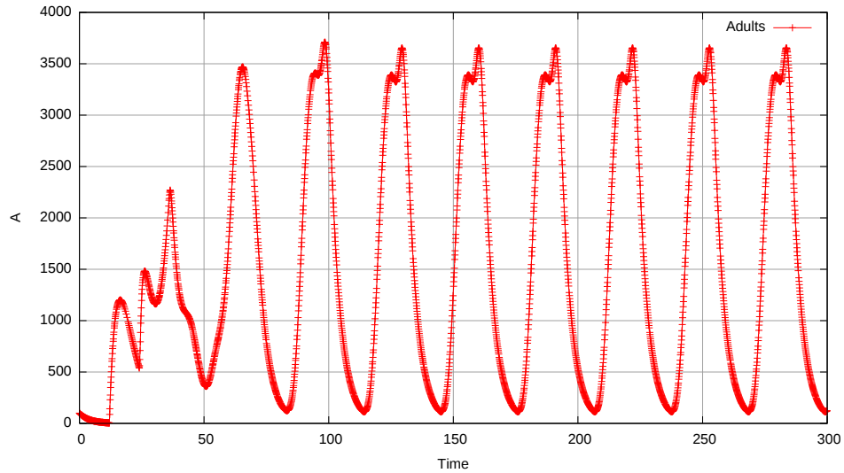
Blowfly DDE model
