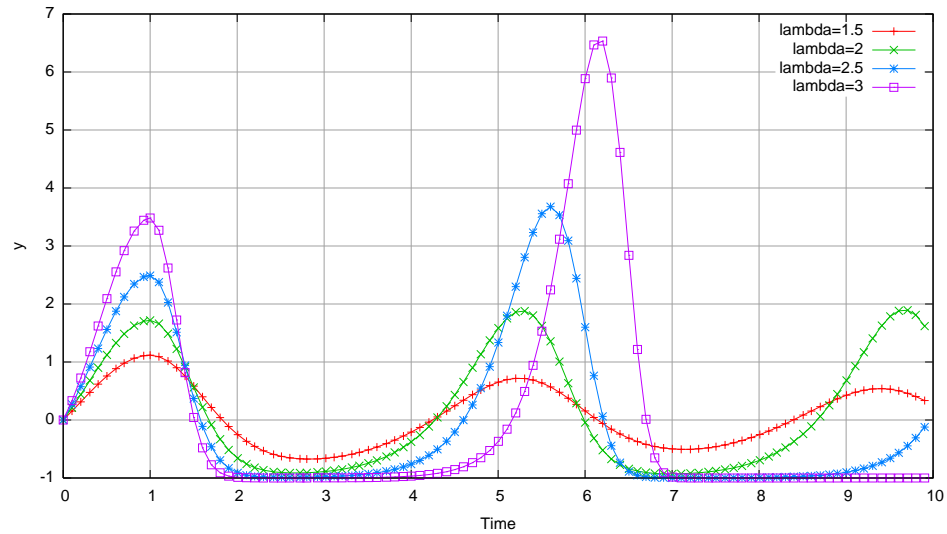
Delay logistic equation
